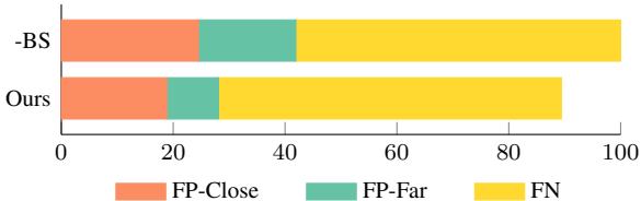
Figure 5. Error analysis of our method: Errors divided into False Positives (FP-Close and FP-Far) and False Negatives (FN). Values are total error pixels relative to the error in the -BS case.
