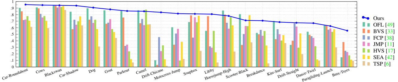
Figure 6. DAVIS Validation : Per-sequence results of region similarity ( \mathcal{J} ).
