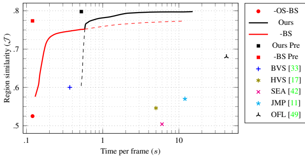
Figure 8. Quality versus timing : Region similarity with respect to the processing time per frame.
