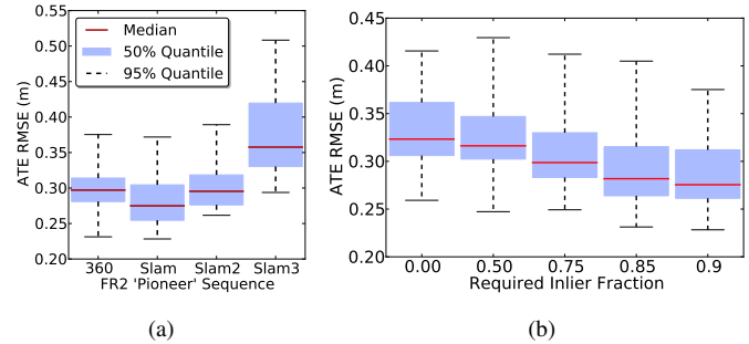
Fig. 9. Evaluation of the accuracy of the presented system on the sequences of the “Robot SLAM” dataset (a). Evaluation of the proposed environment measurement model (EMM) for the “Robot SLAM” scenarios of the RGB-D benchmark for various quality thresholds. The value 0.0 on the horizontal axis represents the case where no EMM has been used. The use of the EMM substantially reduces the error (b).
